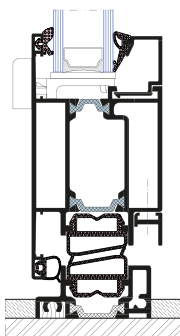
Aluminium threshold
