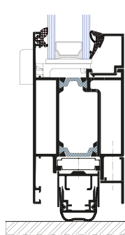
Collapsing threshold strip
