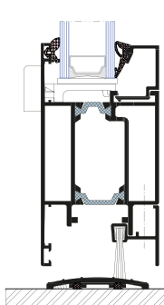
A brush with a threshold strip
