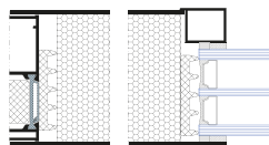
Glazing mounting
