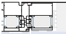
Enamelled glazing variant
