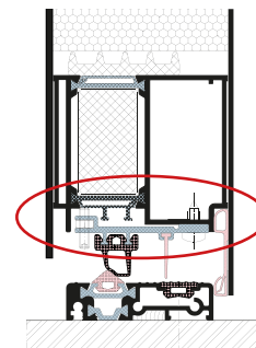
Threshold with adjustable sealing
