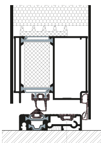
Aluminium threshold
