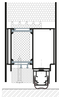
Sloping threshold
