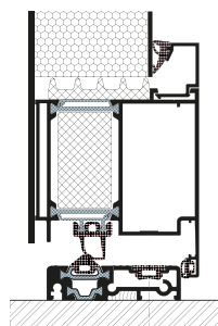
Aluminium threshold
